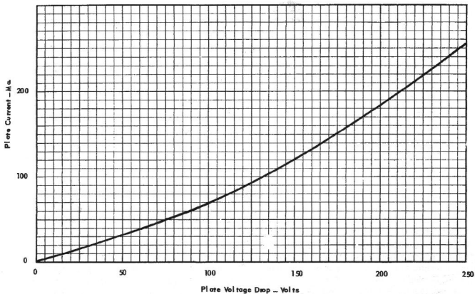
AVERAGE PLATE VOLTAGE DROP
